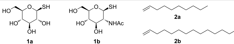
Figure 1: Structure of the \beta -thiols 1a and 1b and of the commercial alkenes 2a and 2b .
