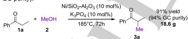
Scheme 2. Scale-up reaction. Reaction conditions: 1a (17.25 mL, 0.124 mol, 1 equiv.), 2 (108 mL, 2.61 mol, 21 equiv.), 65wt%Ni/SiO 2 -Al 2 O 3 (10 mol%, 1.14 g), K 3 PO 4 (10 mol%, 2.64 g), under air, 185°C, in a 300 mL autoclave reactor, 72h.
