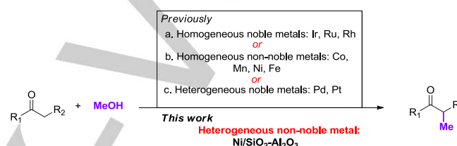
Scheme 1. \alpha -Methylation of ketones with methanol.
