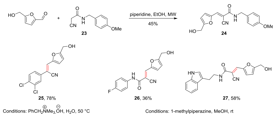
Scheme 9. Condensation of cyanoamides and nitriles derivatives with 5-HMF
