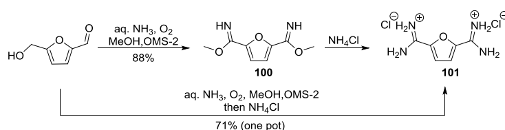
Scheme 39. Transformation of 5-HMF to dicarboximidate and diamidine salt
