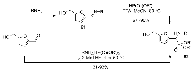
Scheme 26. Synthesis of \alpha -aminophosphonates via Pudovik or Kabachnik-Fields reactions
