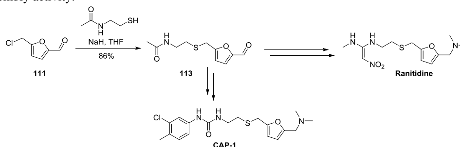
Scheme 43. Synthesis of ranitidine and CAP-1 from 5-HMF
