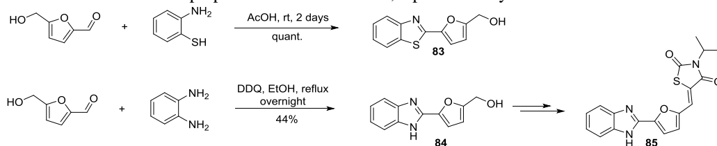
Scheme 34. Synthesis of benzothiazole and benzimidazole derivatives
