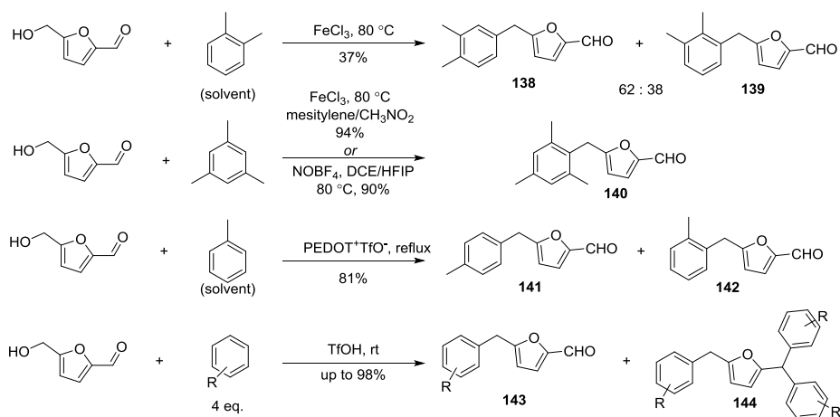
Scheme 56. Friedel–Crafts alkylation of arenes
