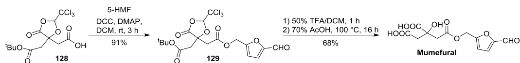
Scheme 51. Synthesis of mumeifural from HMF
