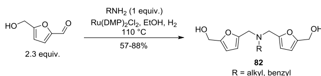
Scheme 33. Double reductive amination
