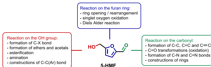
Scheme 1. Overview of 5-HMF chemistry
