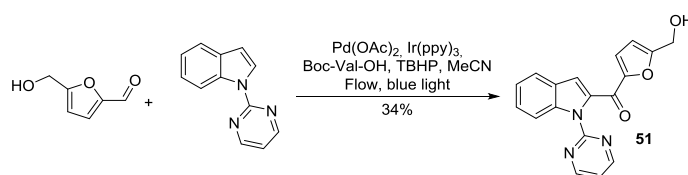
Scheme 21. Acylation of indole using HMF in a photoredox strategy
