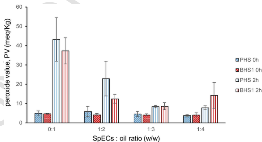
Fig. 6. Comparison of average PVs obtained for irradiated (2h) and non-irradiated (0h) cod liver oil samples after passive encapsulation in PHS SpECs (from Fig. 2) and BHS1 SpECs at various weight ratios. The PVs reported for t = 0 are for samples of \omega -3 oil that had been encapsulated at the appropriate weight ratio, and then extracted from the SpECs without irradiation. Error bars shown are the standard deviation of the average.
