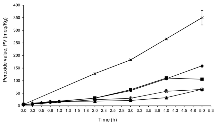
Fig. 11. The change in PV value of samples of a commercial \omega -3 oil supplement against UV irradiation time. The lines shown represent (i) the \omega -3 oil and 3mmol/g of 4-methoxycinnamic acid (crosses); (ii) the \omega -3 oil supplement alone (filled circles); (iii) the \omega -3 oil and 3mmol/g of coumaric acid (squares); (iv) the \omega -3 oil and 3mmol/g of ferulic acid (open circles); (v) a 1:1 w/w mixture of \omega -3 oil encapsulated in base-hydrolysed SpECs, (triangles). Each data point is the average PV from two separate experiments, and the error bars show the standard deviation.
