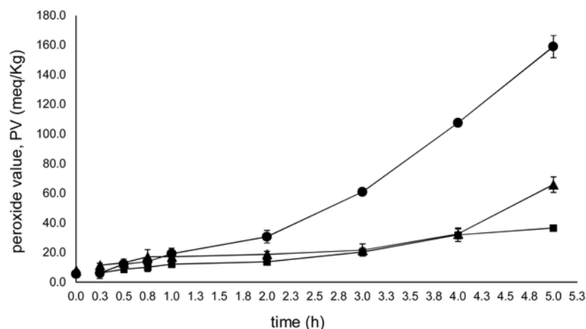
Fig. 7. The change in PV value of samples of a commercial \omega -3 oil supplement against UV irradiation time. The lines shown represent (i) the \omega -3 oil alone (circles); (ii) a 1:1 w/w mixture of \omega -3 oil encapsulated in BHS2 SpECs (triangles); (iii) a 1:1 w/w mixture of \omega -3 oil encapsulated in AHS SpECs (squares). Each data point is the average PV from three separate experiments, and the error bars show the standard deviation.
