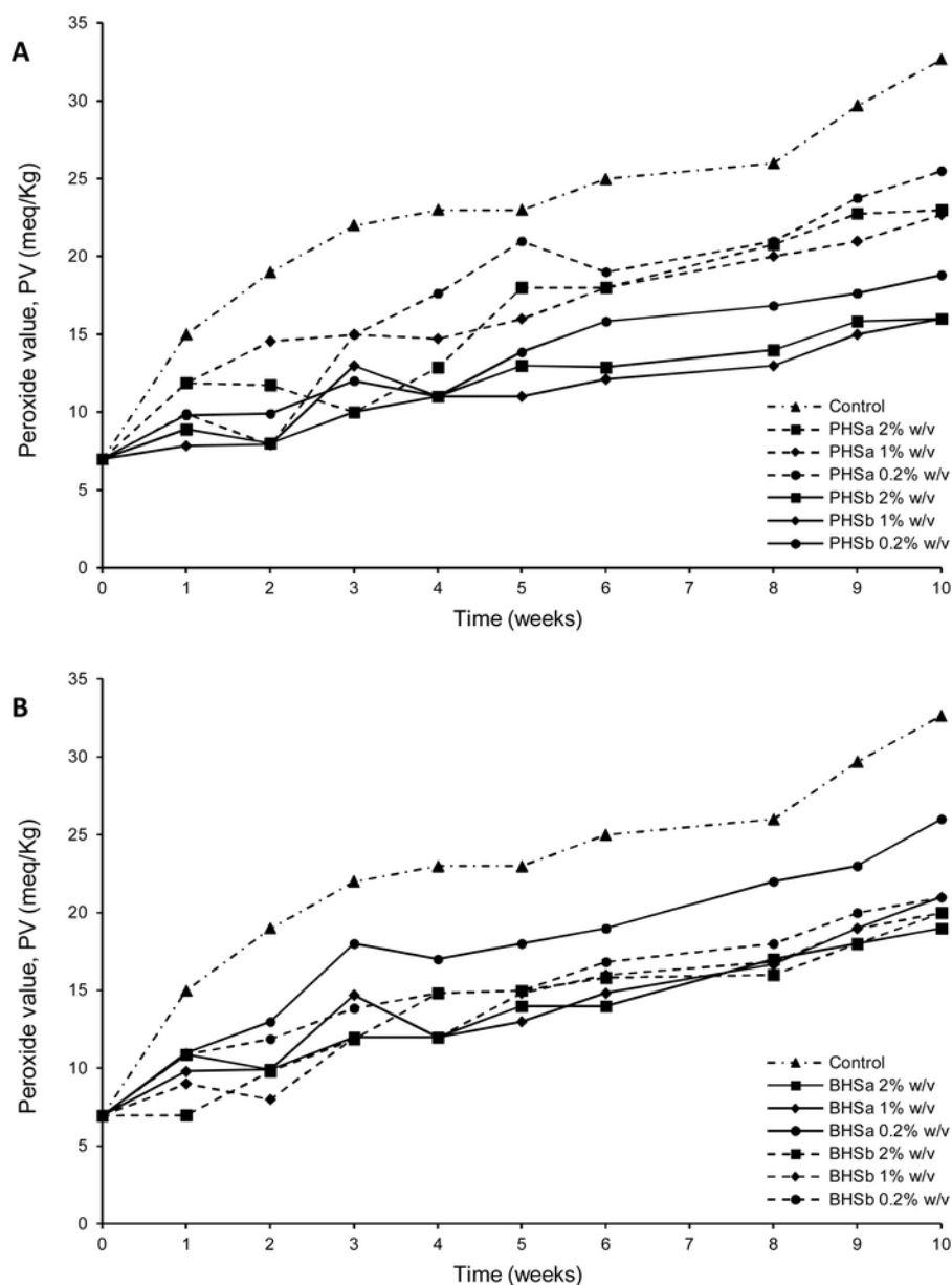
Fig. 8. Progression of PVs over time for \omega -3 oil samples containing either PHS SpECs (A) or BHS1 SpECs (B) at concentration of 2% w/v, 1% w/v, and 0.2% w/v SpECs relative to the \omega -3 oil. On each graph two identically extracted batches of SpECs, labelled a or b, are compared.
