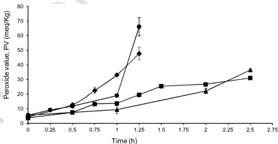
Fig. 10. The change in PV value of samples of a commercial \omega -3 oil supplement against UV irradiation time. The lines shown represent (i) the \omega -3 oil supplement alone (circles); (ii) a 1:1 w/w mixture of \omega -3 oil encapsulated in phosphoric acid-hydrolysed SpECs, PHS, (triangles); (iii) an intimate mixture of \omega -3 oil and 3 mmol/g of 2,6-di- tert -butyl-4-methylphenol [butylated hydroxytoluene, BHT] (squares); (iv) a 1:1 w/w mixture of \omega -3 oil encapsulated in methylated phosphoric acid-hydrolysed SpECs, Me-PHS, (diamonds). Each data point is the average PV from three separate experiments, and the error bars show the standard deviation.
