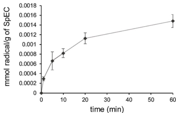
Fig. 9. Time profile of the mmol of DPPH radicals quenched per gram of PHS SpECs over the course of 60 min ( n = 5 ).
